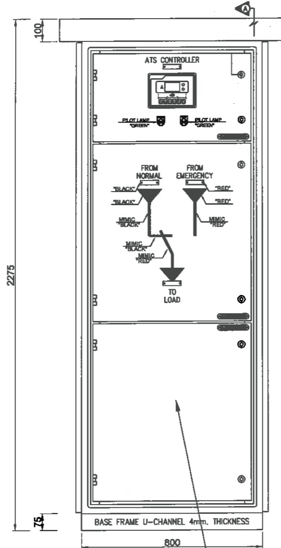
FRONT WITHOUT COVER-1
