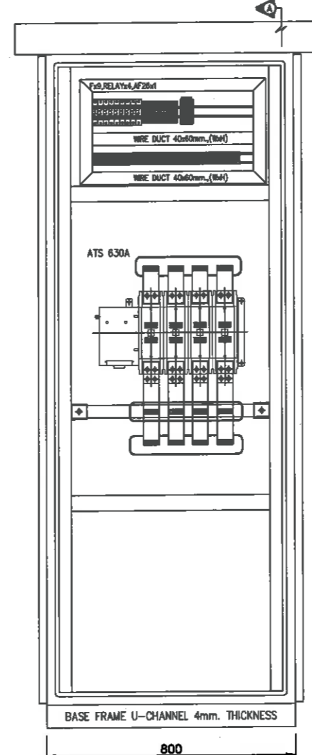
FRONT WITHOUT COVER-2
