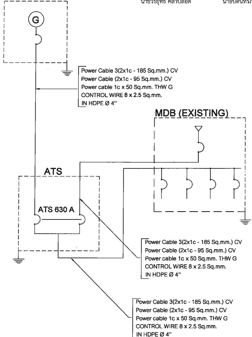
SINGLE LINE DIAGRAM
