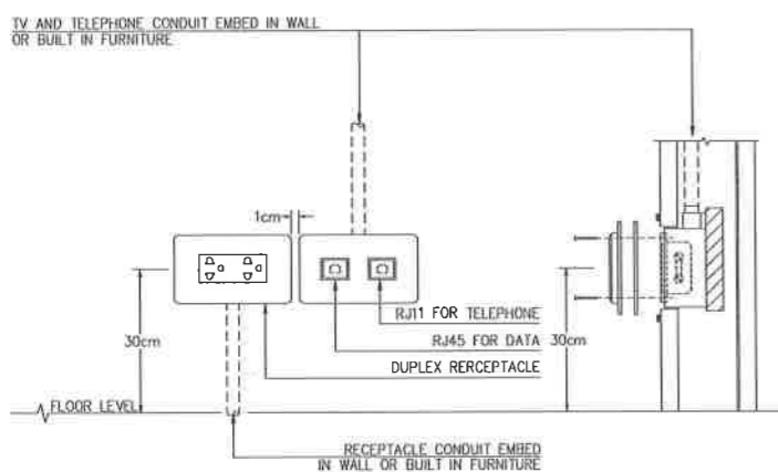
04 RECEPTACLE, TV, TELEPHONE INSTALLATION NTS
