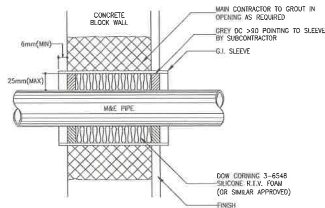
08 SLEEVE THROUGH FIRE WALL-ABOVE CEILING NTS
