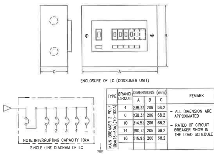
02 CONSUMER UNIT NTS
