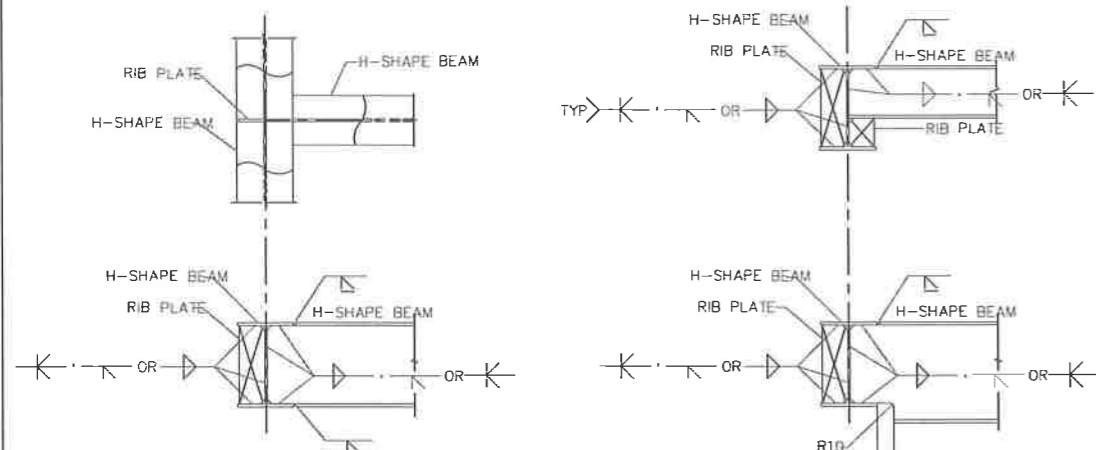
H-SHAPE TO H-SHAPE (COLUMN TO BEAM)
