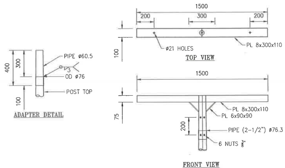
SUPPORT LIGHTING DETAIL
