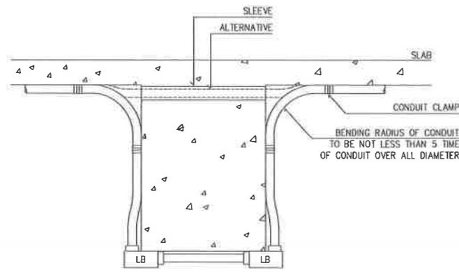
01 TYPICAL CONDUIT RUN OVER SIDE OF BEAM NTS
