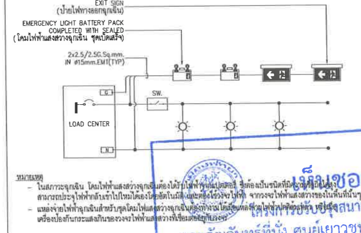
09 DIAGRAM FOR EMERGENCY BATTERY LIGHT
