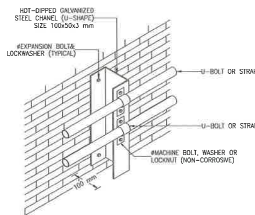
05 TYPICAL WALL MOUNTING CONDUIT SUPPORT NTS
