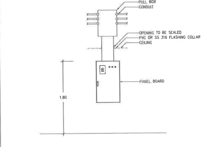
03 DETAIL FOR CONDUIT , BOX , WIREWAY AND PANEL BOARD INSTALLATION
