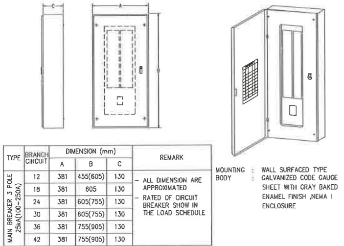
01 LOAD CENTER (MAIN BREAKER TYPE) NTS
