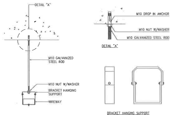
04 WIREWAY BRACKET HANGING SUPPORT NTS
