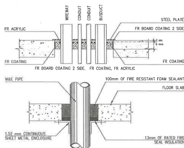
07 CONDUIT OR WIREWAY OR BUSDUCT THROUGH FLOOR NTS
