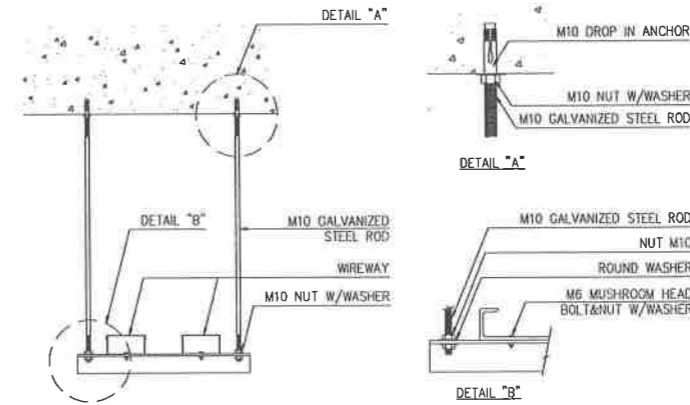
03 WIREWAY BRACKET HANGING SUPPORT NTS
