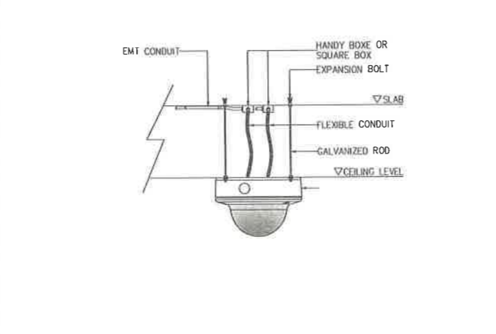
08 INSTALLATION DETAIL FOR FIXED DOME CAMERA NTS
