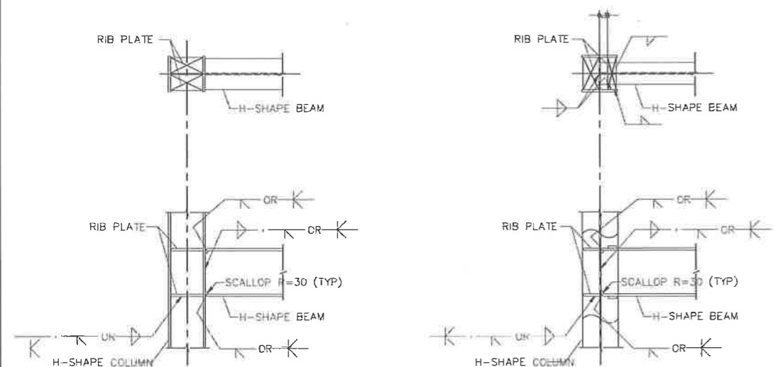
H-SHAPE TO H-SHAPE (COLUMN TO BEAM)
