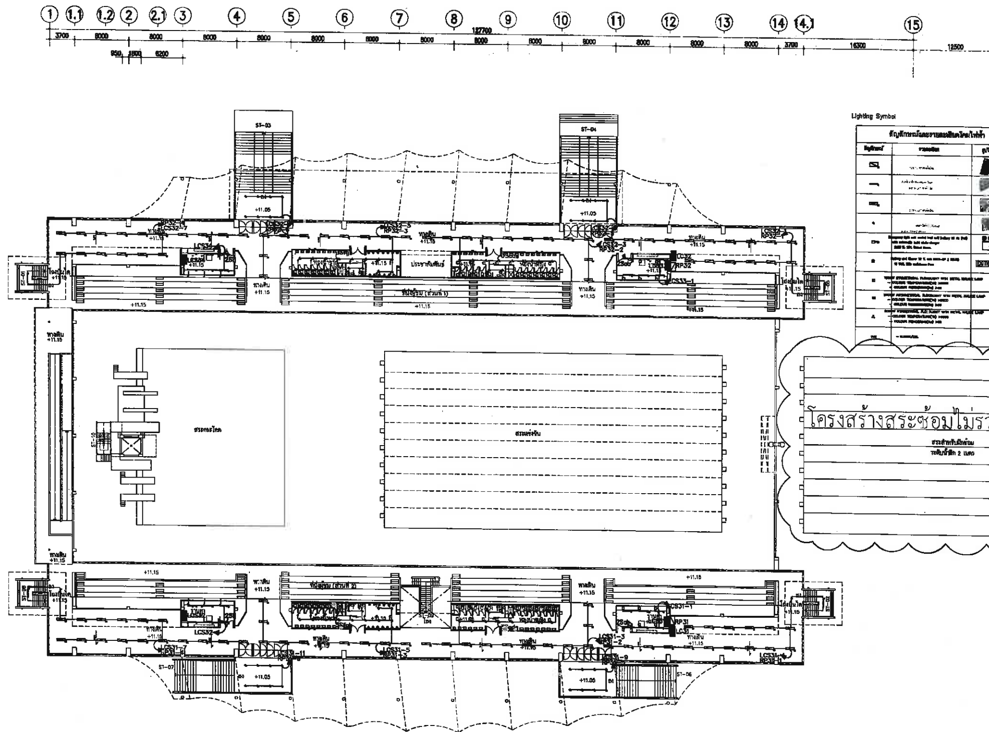
LIGHTING FIXTURE LAYOUT 3rd PLAN SCALE 1:250 AT A1 1:500 AT A3
