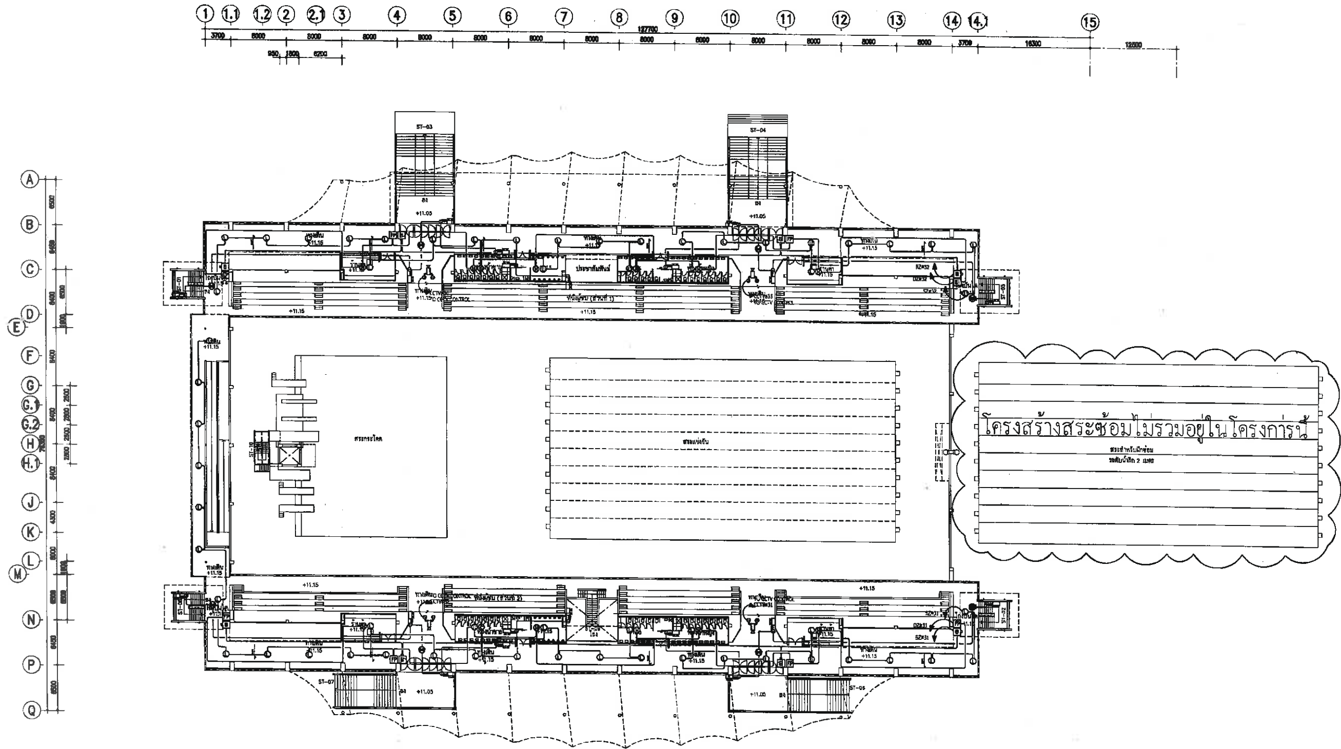
FIRE ALARM, SOUND, CCTV & EMERGENCY LIGHT SYSTEM 3rd PLAN SCALE 1:250 AT A1 1:500 AT A3
