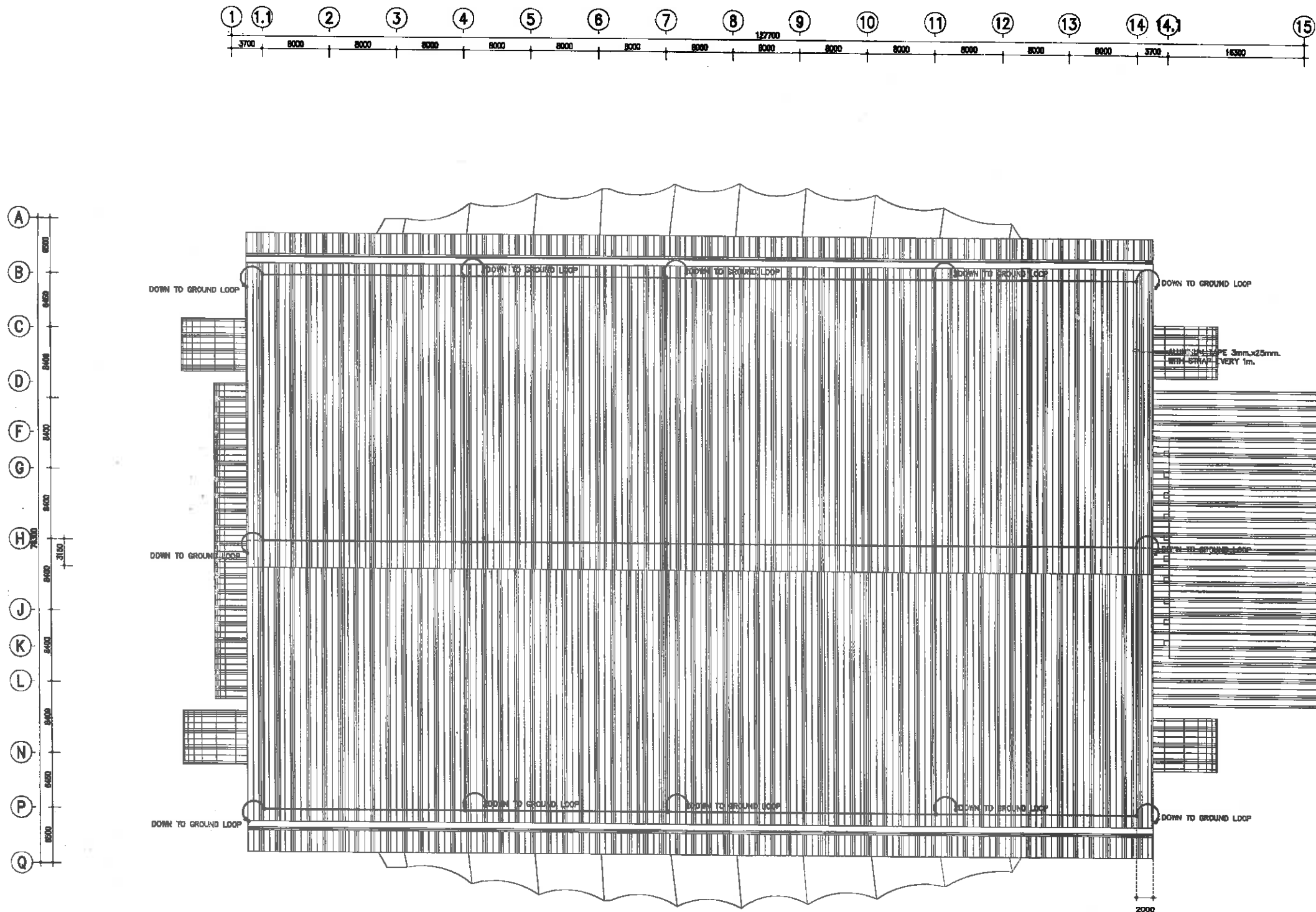
LIGHTNING PROTECTION SYSTEM ROOF PLAN SCALE 1:250 AT A1 1:500 AT A3
