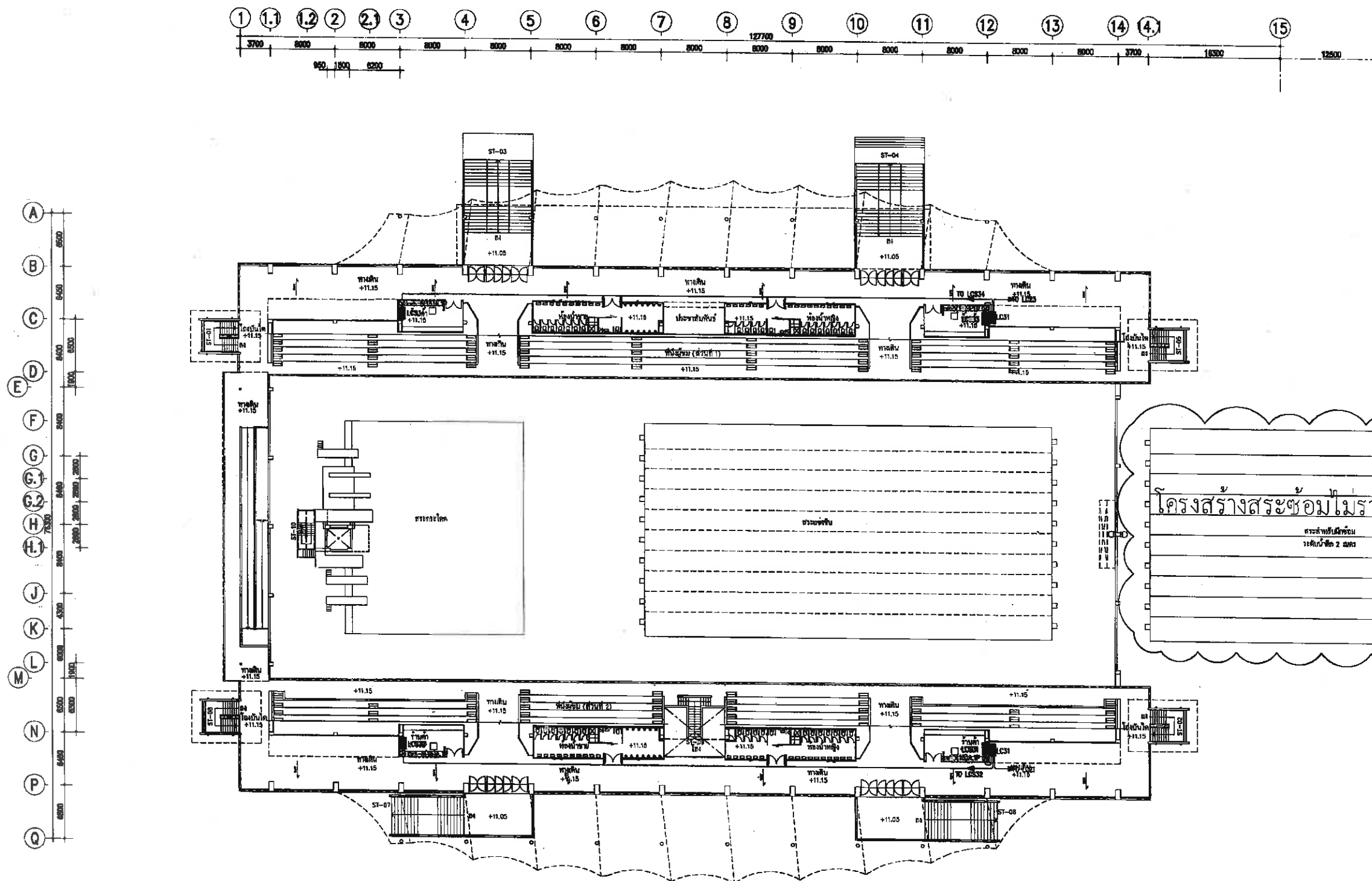
ELECTRICAL POWER FEEDER SYSTEM 3rd PLAN SCALE 1:250 AT A1 1:500 AT A3
