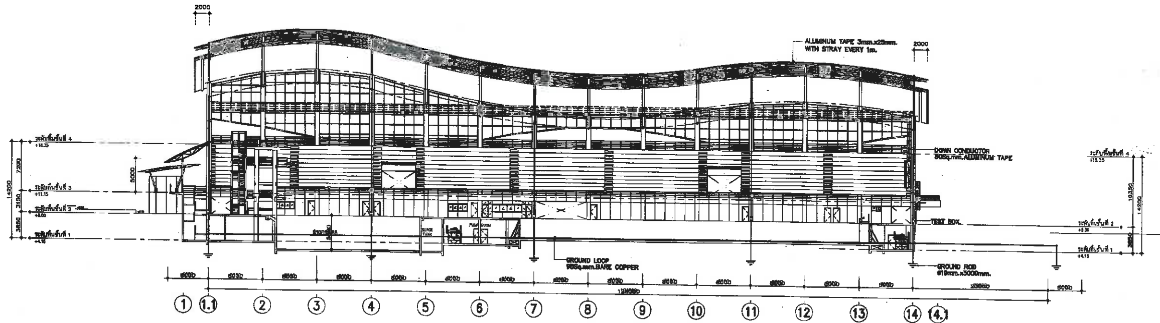
GROUNDING & LIGHTNING PROTECTION SYSTEM SECTION 1 PLAN SCALE 1:200 AT A1 1:500 AT A3
