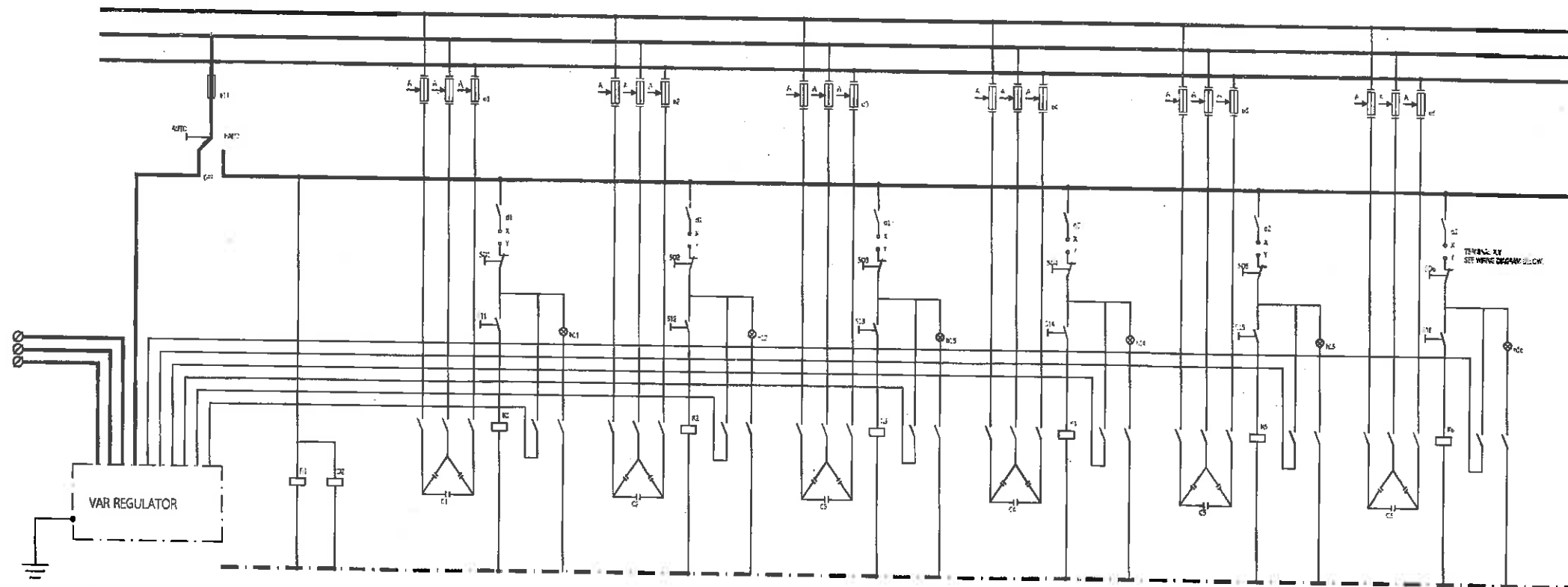
VAR REGULATOR WIRING DIAGRAM (TYPICAL)
