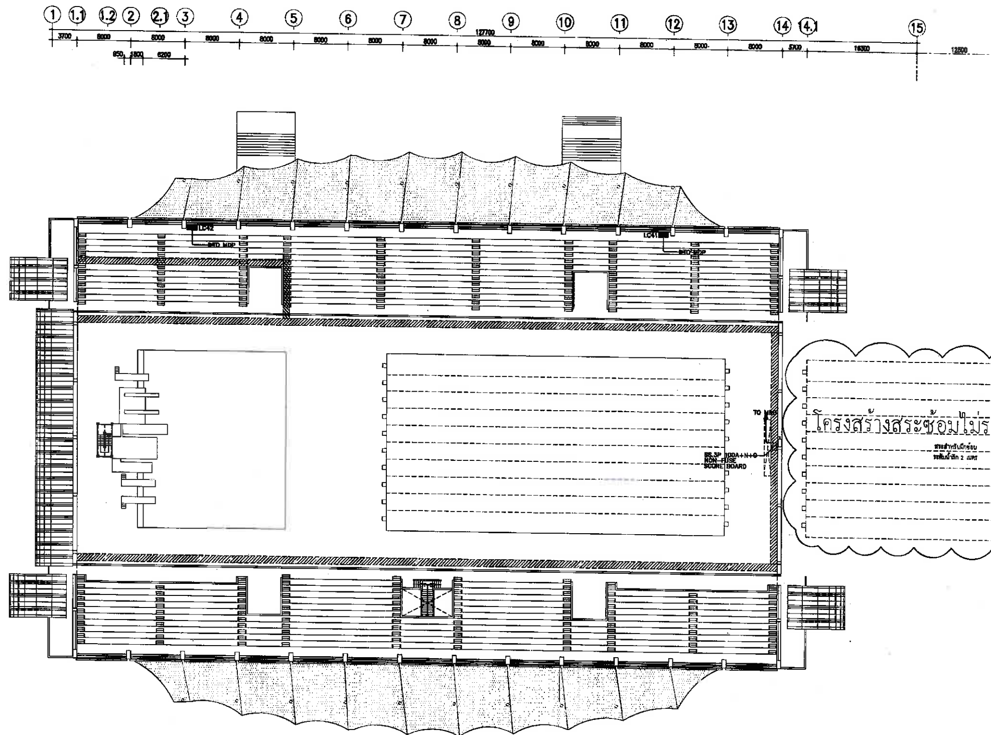
ELECTRICAL POWER FEEDER SYSTEM 4th PLAN SCALE 1:250 AT A1 1:500 AT A3
