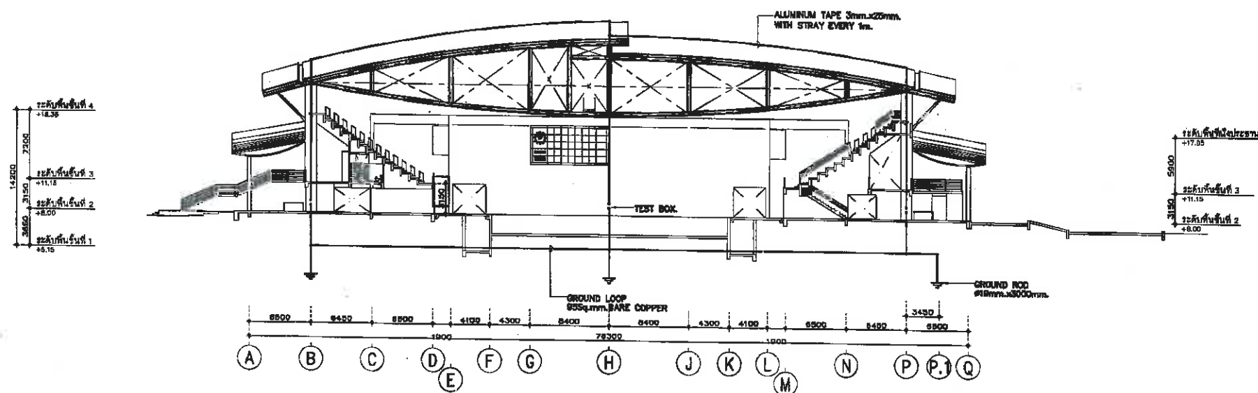
GROUNDING & LIGHTNING PROTECTION SYSTEM SECTION 2 PLAN SCALE 1:200 AT A1 1:500 AT A3
